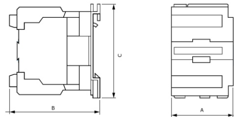
CJX2-40/50/65/80/95
