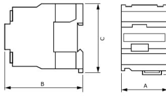
CJX2-25/32
