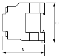
CJX2-09/12/18
